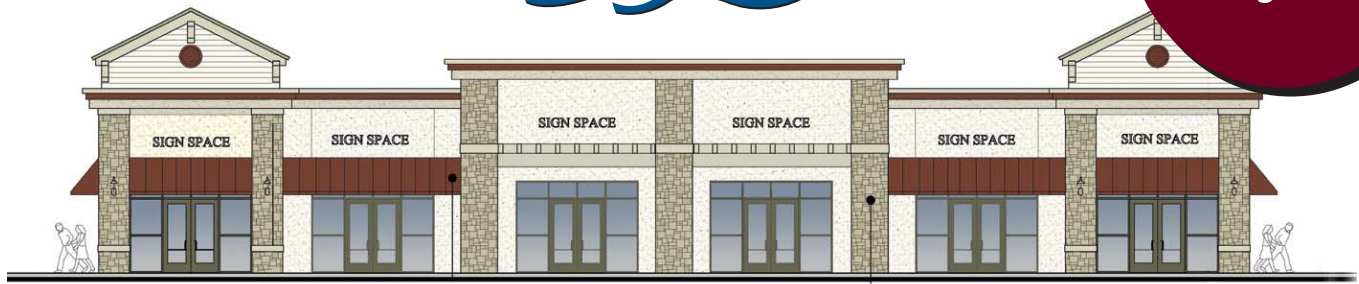
SOUTH ELEVATION (BLDG. B) SCALE: 1/8" = 1'-0"
